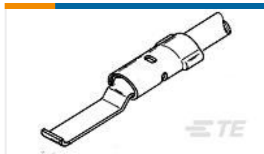
TE Part #151467 22-16 PIDG LIPPED BLADE EXP.1
