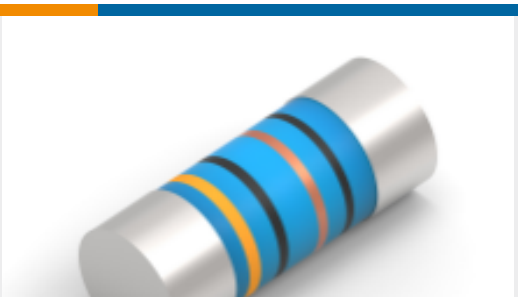
TE Part #2-2176316-5 MELF SMA_A 10K 0.1% 15PPM 0207 1W
