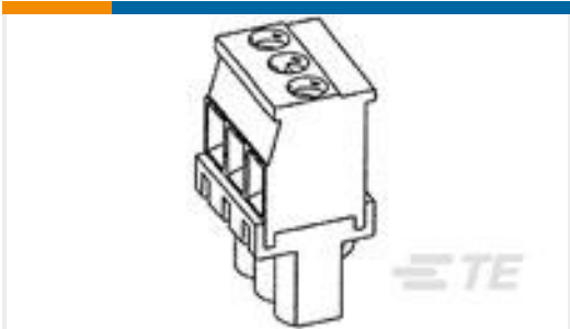
TE Part #1-1986370-0 Str Plug, 3.5mm, Green, RH, 10
