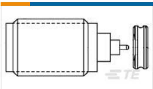
TE Part #1053254-1 2058 5278 00 SMA FEEDTHRU JACK, SEALED
