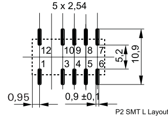
SMT, long terminals
