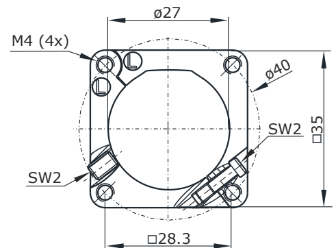
Main Dimensions flange
