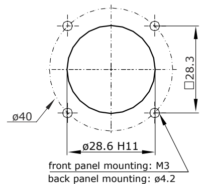
Mounting Hole
