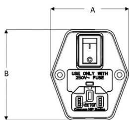
Class II, IEC 60320 C18
