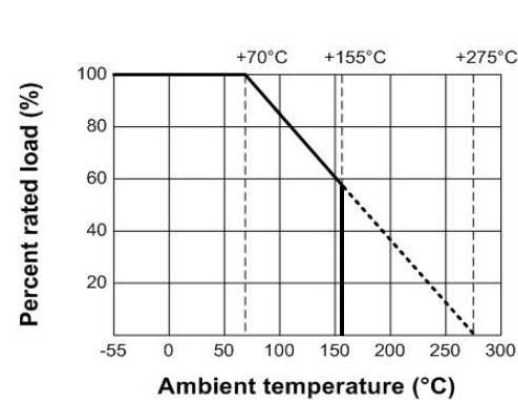
Derating Curve
