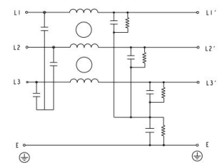
TYPICAL CIRCUIT DIAGRAM
