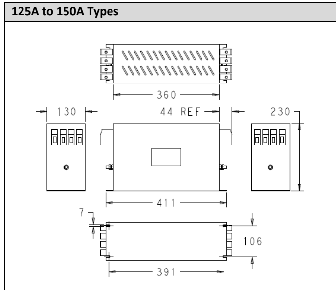
Case Dimensions – Din Rail Mount
