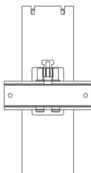
HORIZONTAL MOUNT
