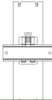
HORIZONTAL MOUNT
