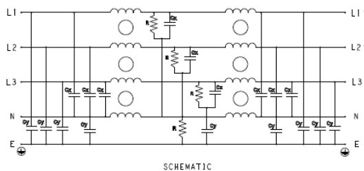
Typical Circuit Diagram
