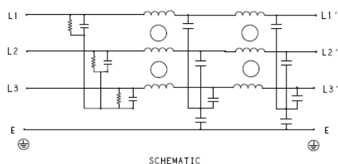
Typical Circuit Diagram
