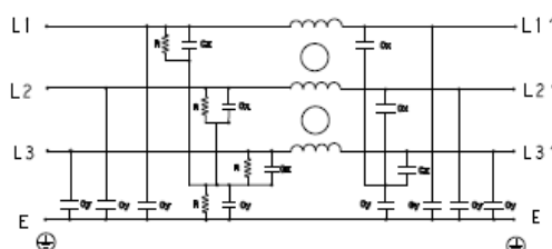
SCHEMATIC
