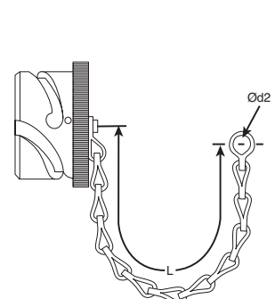
CIRB-**-E-PCAK (with sash chain)
