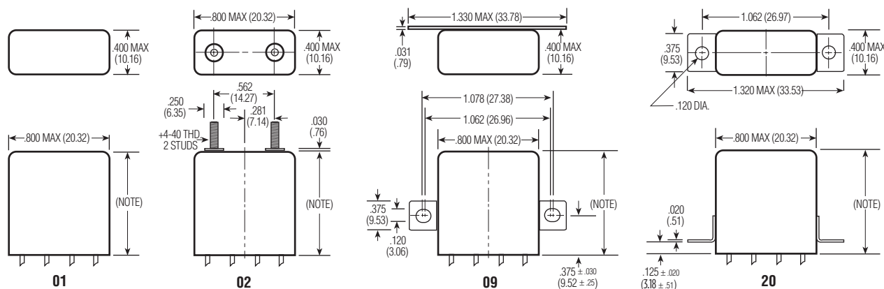
Mounting Styles
