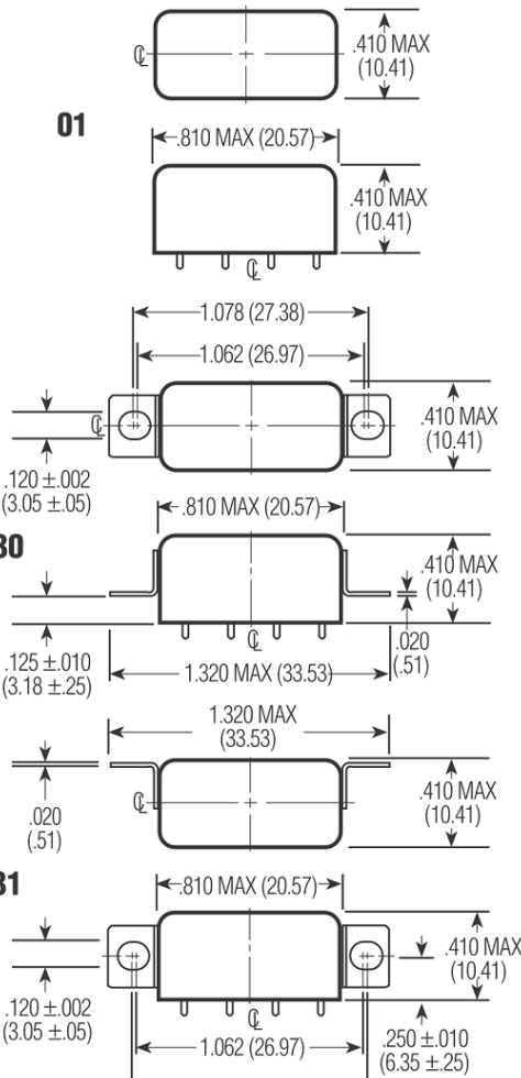
Mounting Styles
