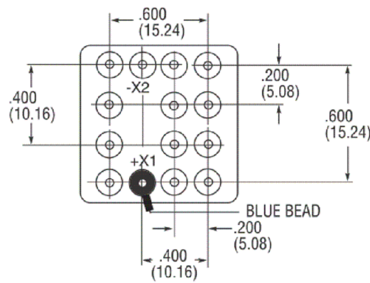
TERMINAL VIEW
