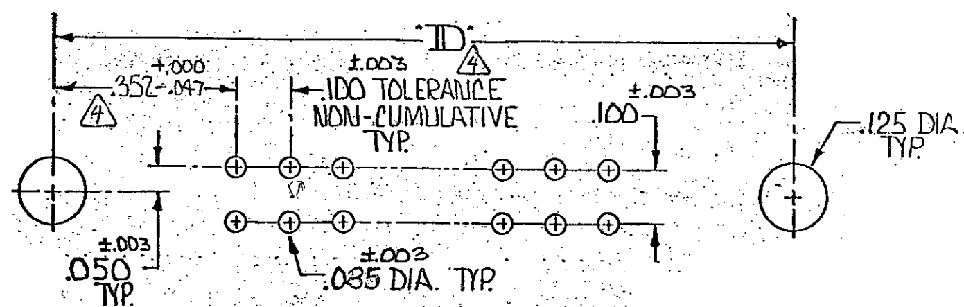
RECOMMENDED HOLE LAYOUT
