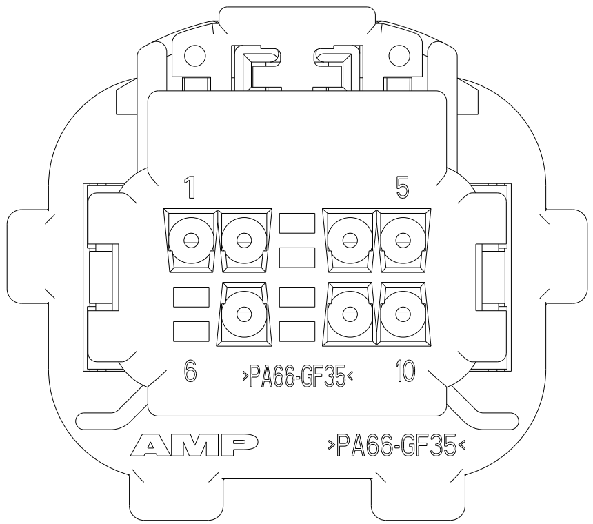
VIEW SHOWS COVER, FOR 2-638517-1
