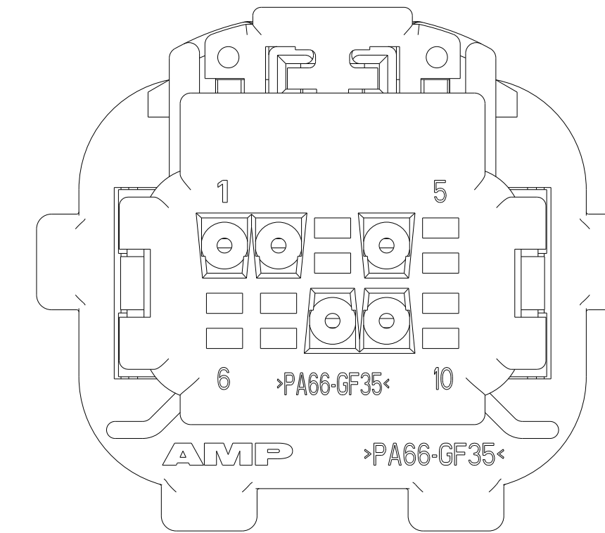
VIEW SHOWS COVER, FOR 3-638517-1
