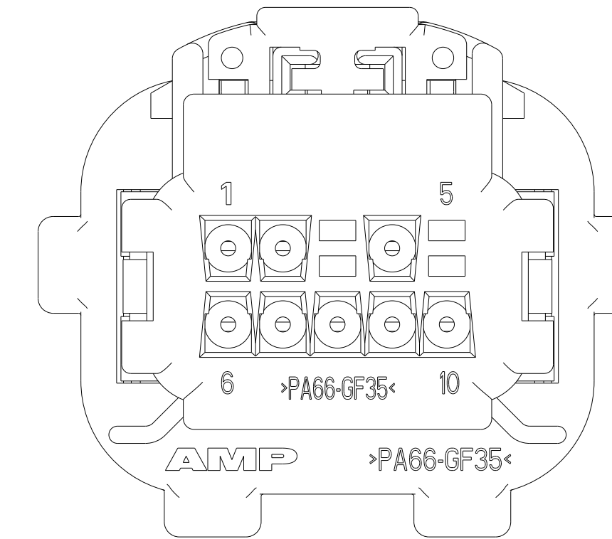
VIEW SHOWS COVER, FOR 2-638517-9
