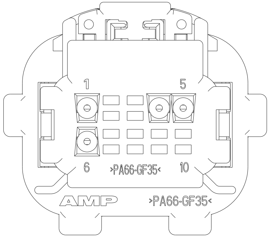
VIEW SHOWS COVER, FOR 2-638517-6
