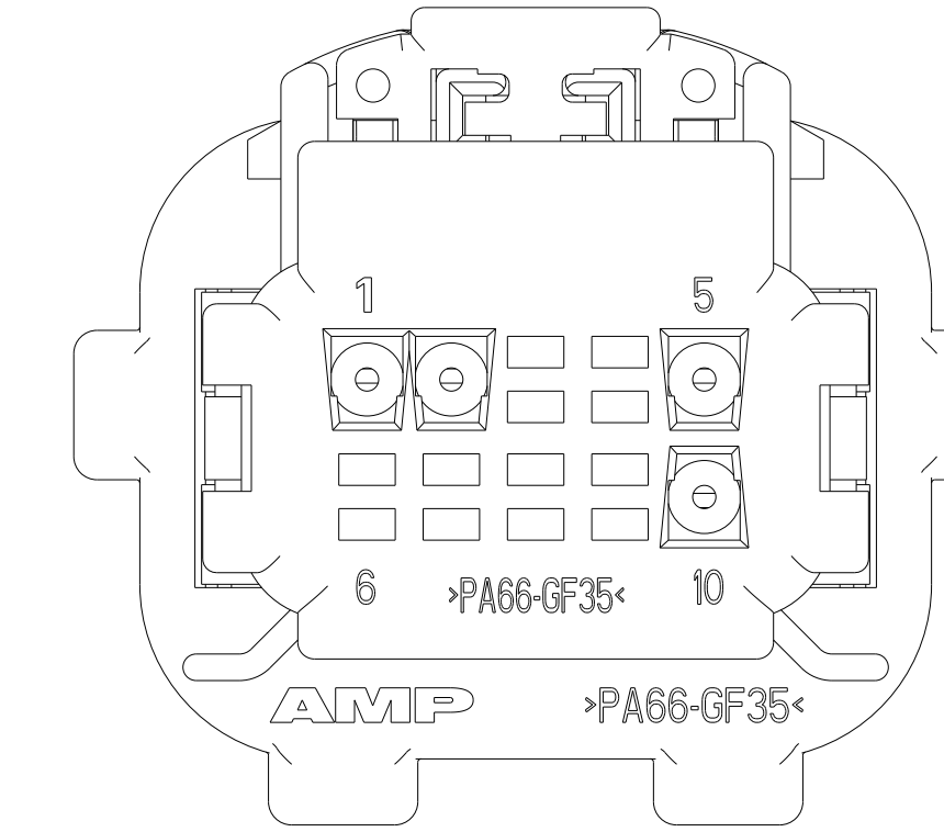
VIEW SHOWS COVER, FOR 2-638517-7
