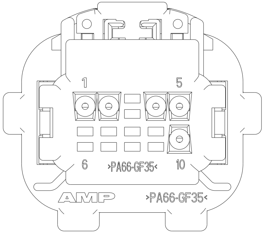
VIEW SHOWS COVER, FOR 2-638517-5
