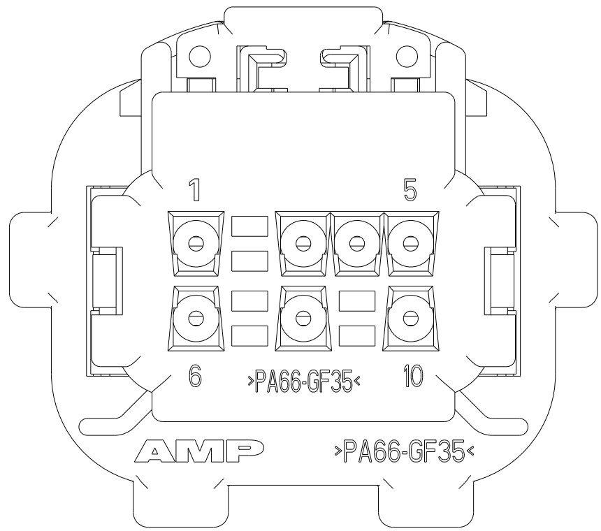
VIEW SHOWS COVER, FOR 2-638517-4 & 5-638517-4
