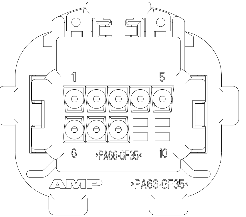
VIEW SHOWS COVER, FOR 2-638517-8
