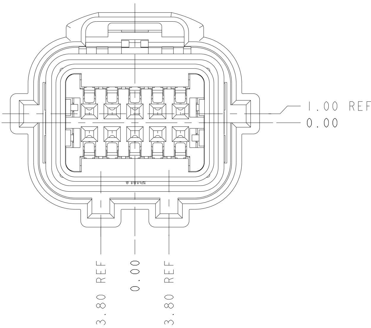
KEY CODE "C" (APPLIES TO -7 ONLY) SCALE 4:1
