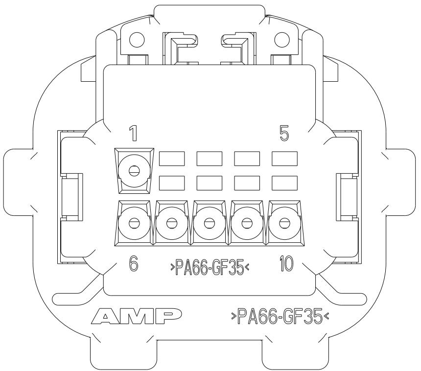
VIEW SHOWS COVER, FOR 3-638517-0
