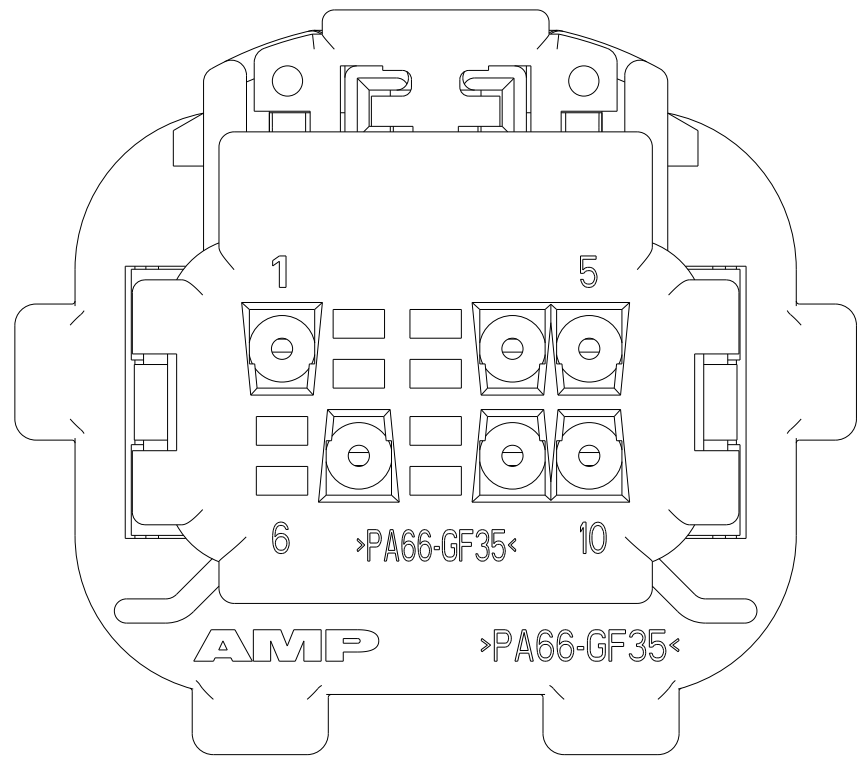
VIEW SHOWS COVER, FOR 2-638517-2
