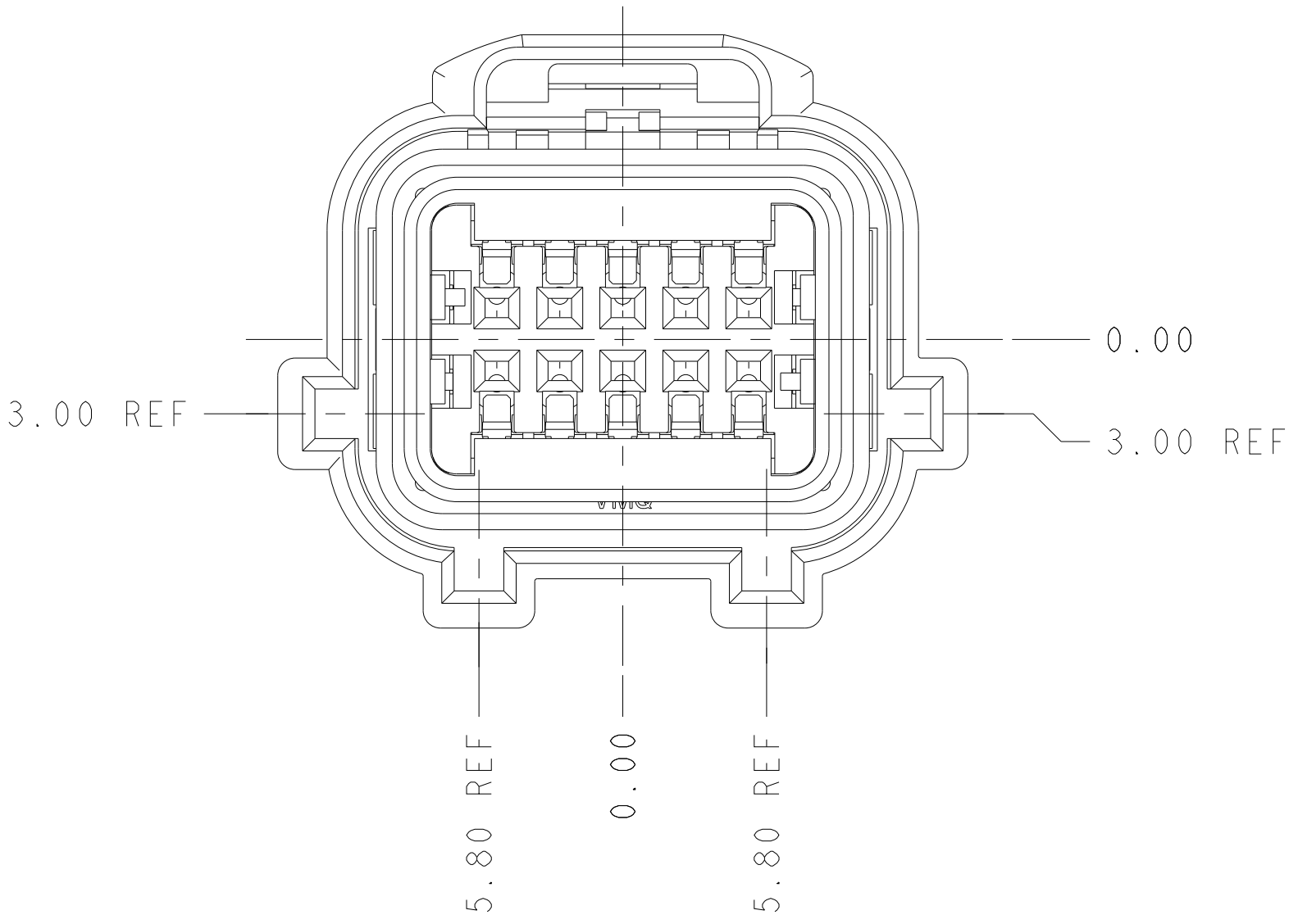
KEY CODE "B" (APPLIES TO -6 ONLY) SCALE 4:1
