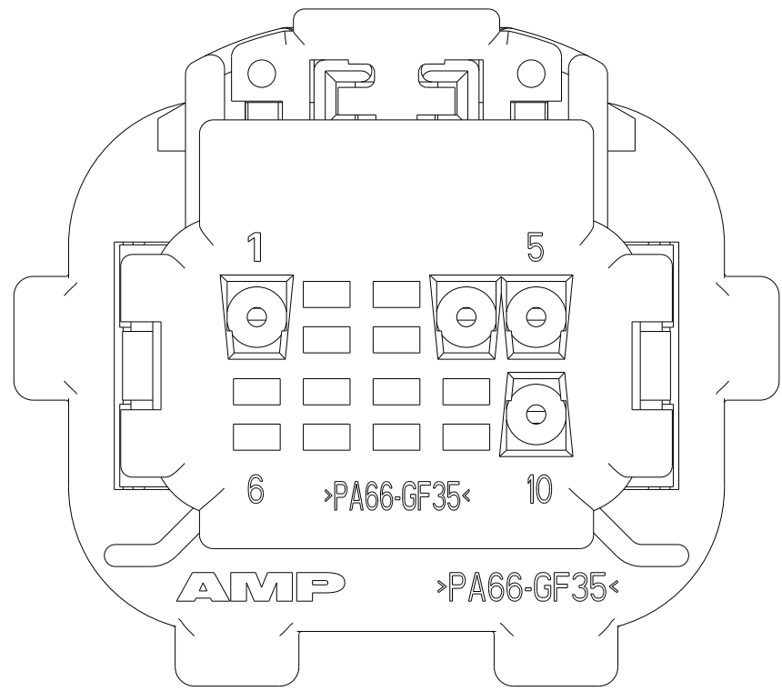
VIEW SHOWS COVER, FOR 2-638517-3
