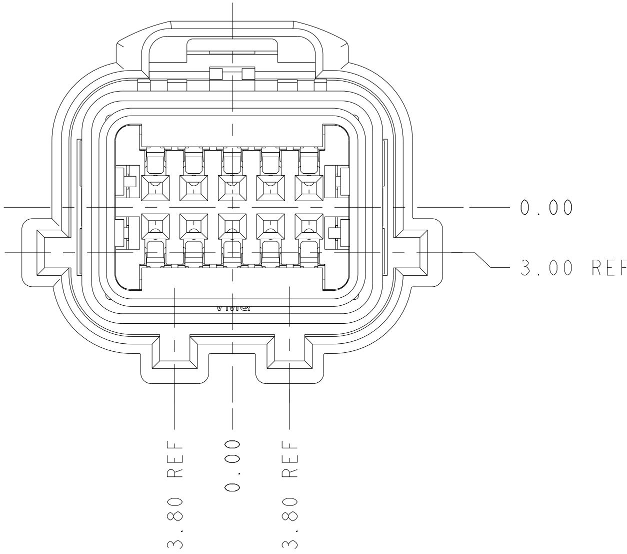
KEY CODE "D" (APPLIES TO -8 ONLY) SCALE 4:1
