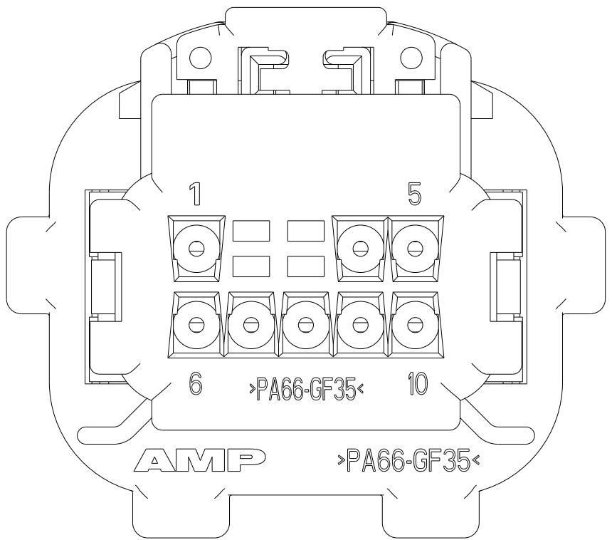
VIEW SHOWS COVER, FOR 3-638517-2
