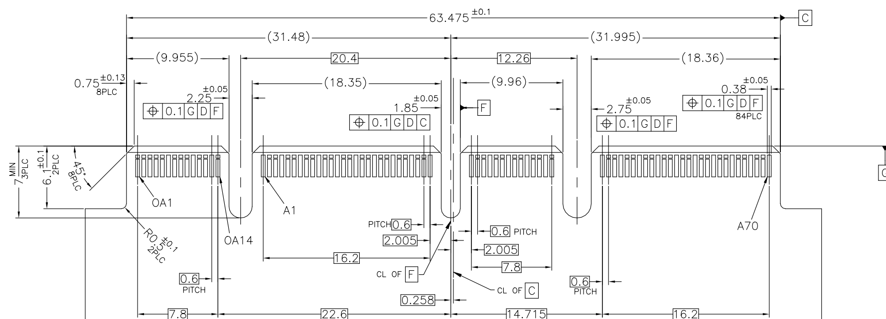
VIEW B-B
