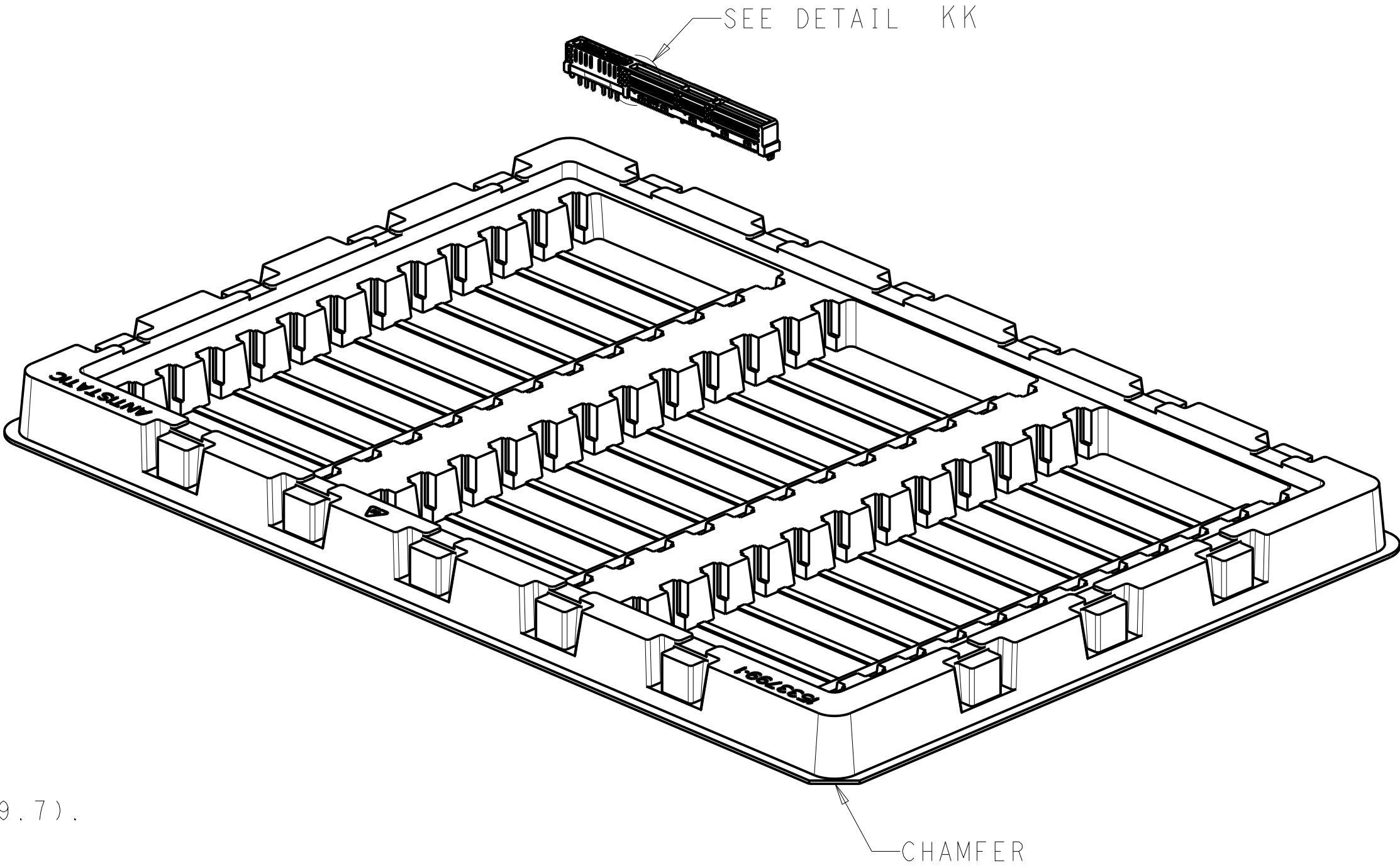
FIGURE 1 SOFT TRAY PACKAGING 2338718-1 AND 2338718-2 SCALE 3:4
