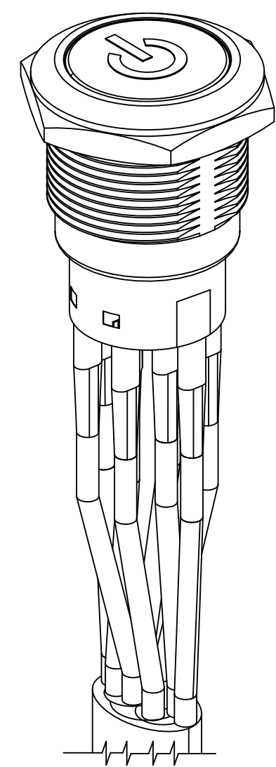
ASSEMBLED VIEW
