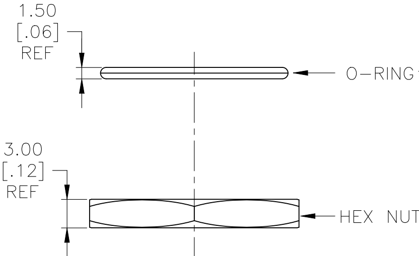
EXPLODED VIEW
