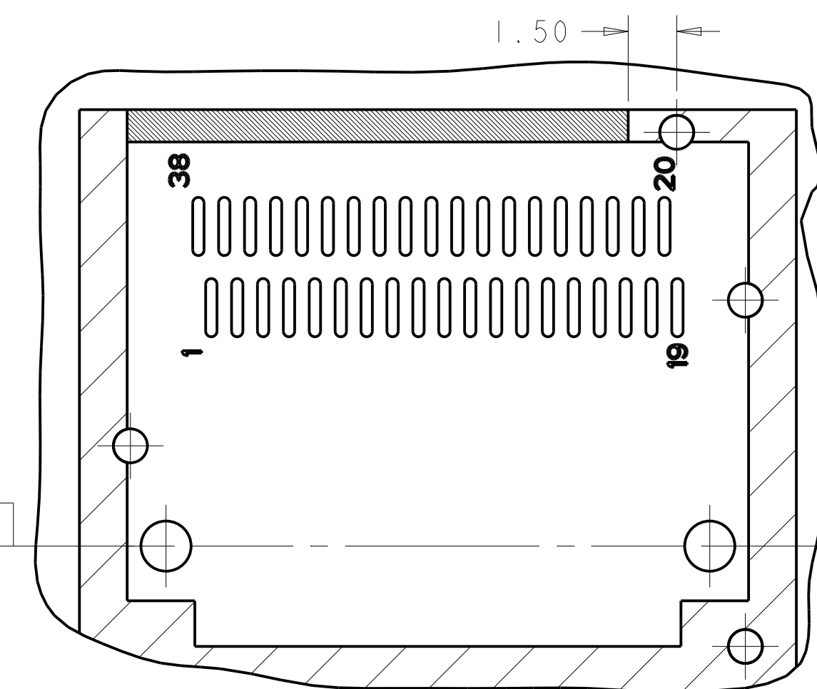
RECOMMENDED PCB LAYOUT SINGLE TYPE OF 1 REAR HOLES OF LEGS PCB TOLERANCE: \pm 0.05 SCALE 6:1
