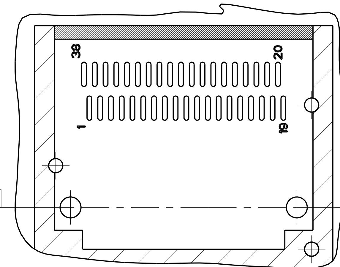
RECOMMENDED PCB LAYOUT SINGLE TYPE OF 0 REAR HOLES OF LEGS PCB TOLERANCE: \pm 0.05 SCALE 6:1
