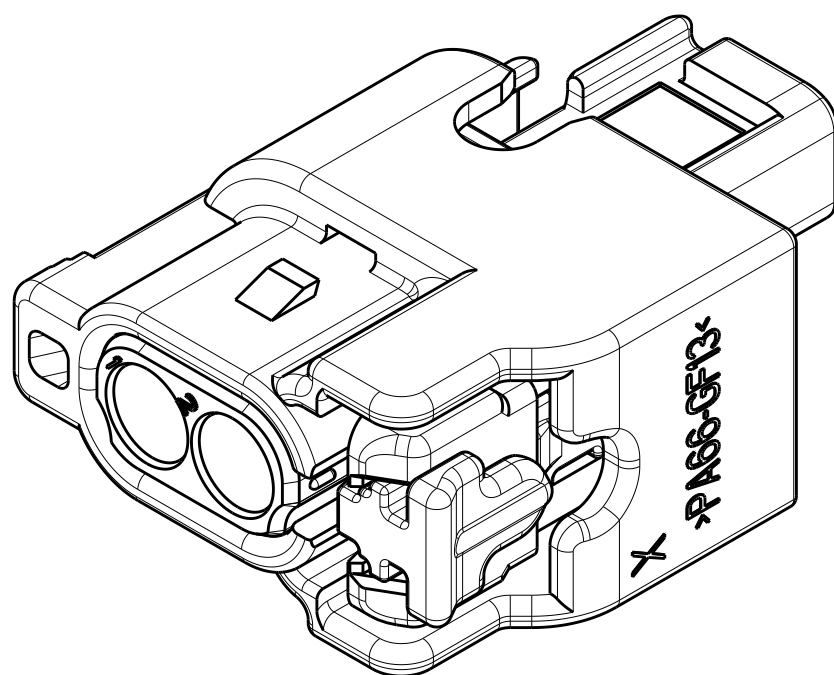
ISOMETRIC VIEWS 2098641-6
