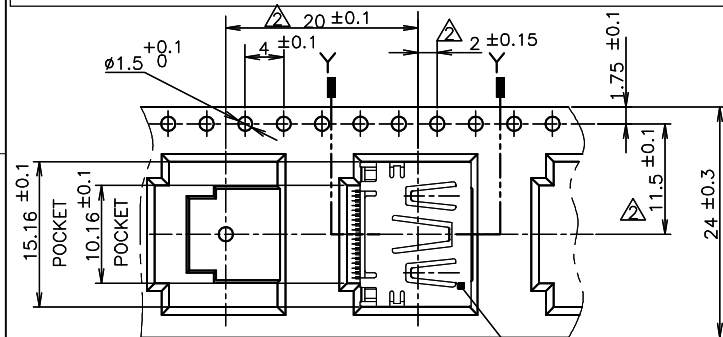
DETAIL X
