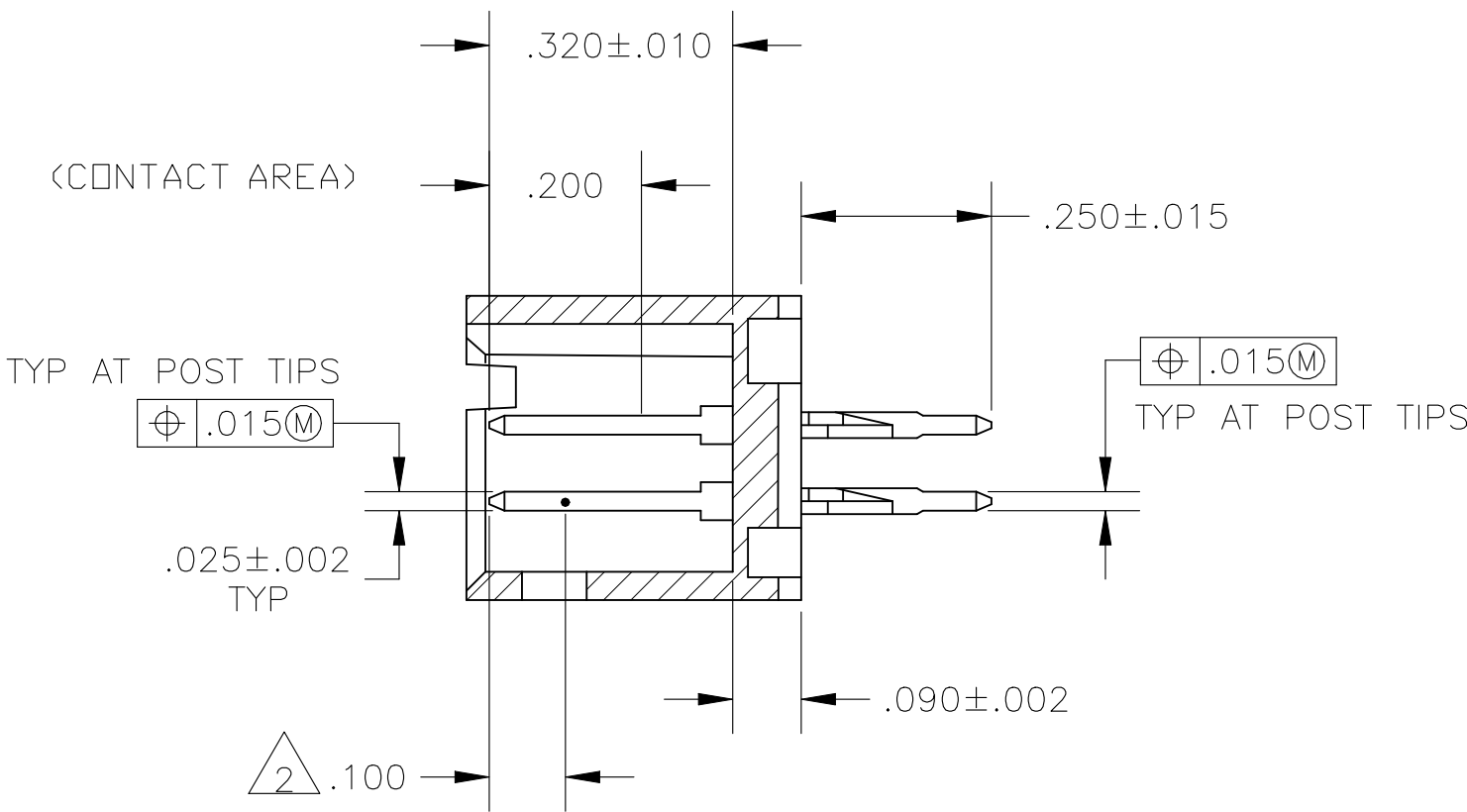
SECTION X-X
