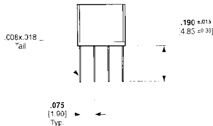
534175 Series
