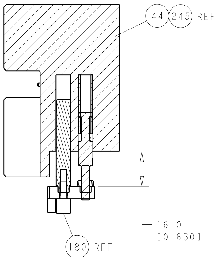
HOLDDOWN SET-UP
