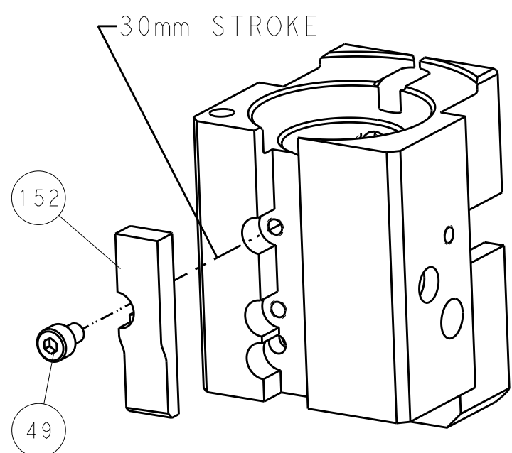
AIR FEED
