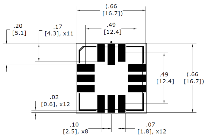
PC board solder pad layout and dimensions
