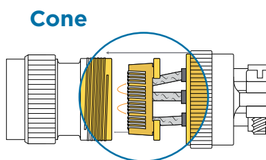
Braid/Pigtails clamped between cones Used on: 64/308/HexaShield Series
