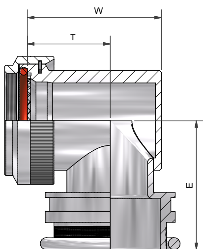
90° BACKSHELL
