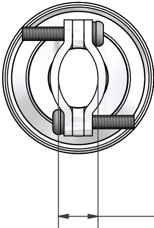
M: MINIMUM CLAMPING DIAMETER
