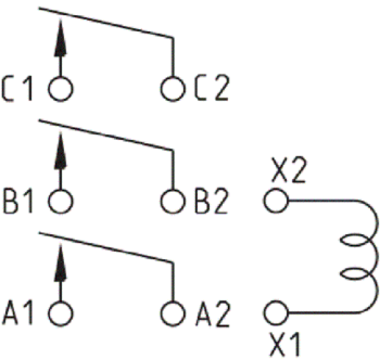
DC Nonsuppressed and AC Coils
