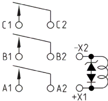
DC Suppressed Coils
