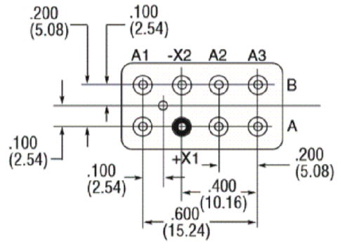
TERMINAL VIEW
