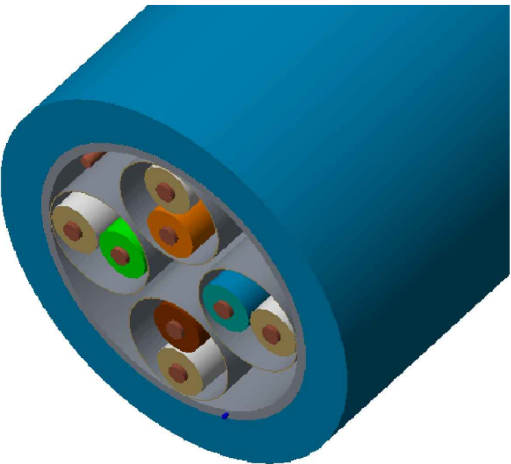
SECTIONAL ISO VIEW OF THE CABLE
