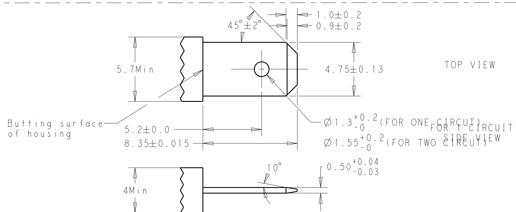
FOR 1 CIRCUIT SIDE VIEW
