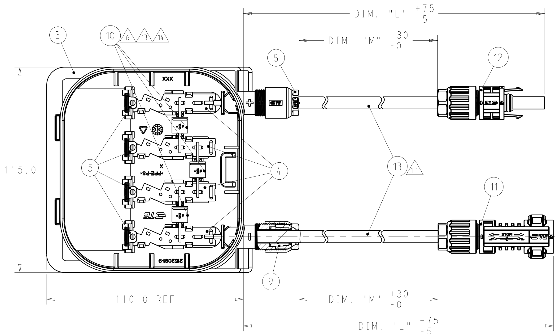
LID ASSEMBLY SHOWN WITHOUT COVER FOR REFERENCES ONLY
