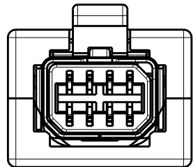
MATING SHAPE : TYPE II 1-2201855-1/-2 SCALE 3:1
