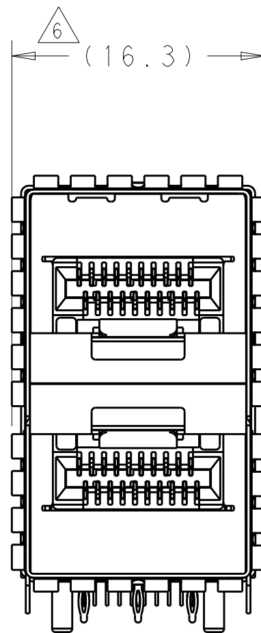
2198318-5 THRU 2198318-8, 1-2198318-9, 2-2198318-0 EMI SPRINGS ONLY SCALE 3:1
