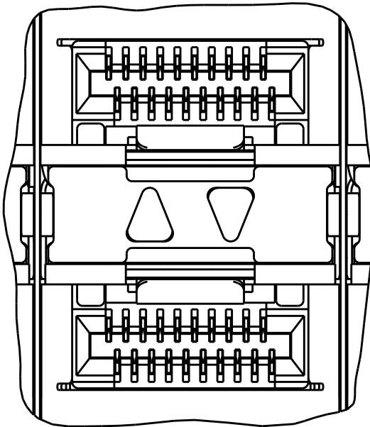
INNER LIGHT PIPES 2180324-3, 2180324-7 SCALE 4:1
