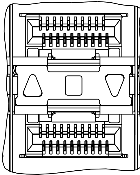
CENTER/REVERSED OUTER 1-2180324-7, 1-2180324-9 SCALE 4:1
