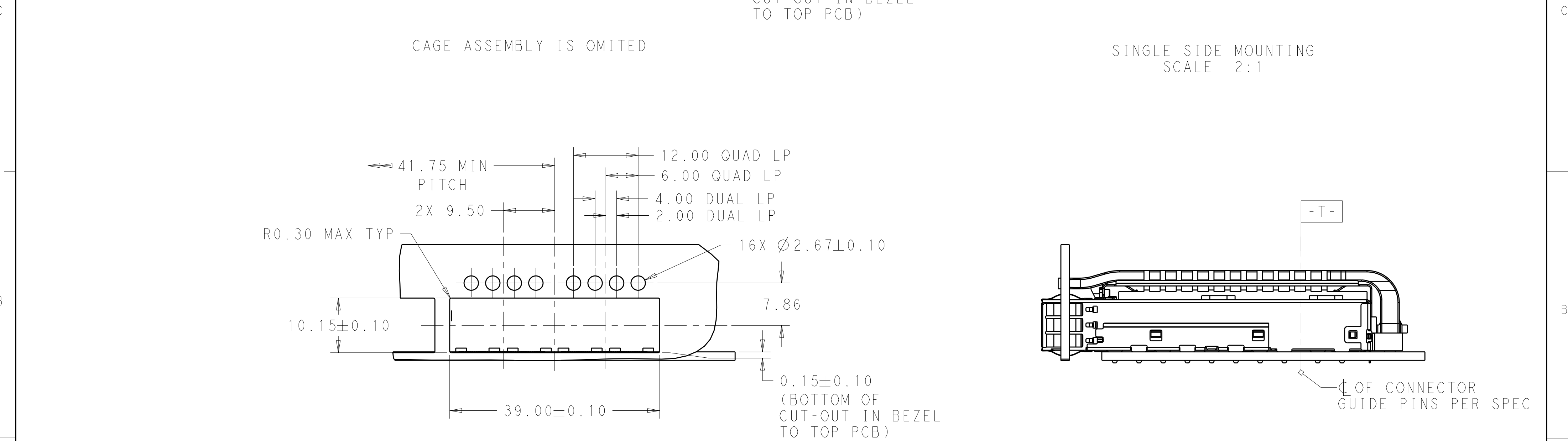
SINGLE SIDE MOUNTING SCALE 2:1
