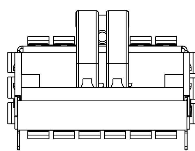
BACK VIEW OF 2170773-3 SCALE 4:1
