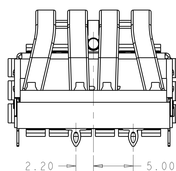
BACK VIEW OF 2170773-4 SCALE 4:1
