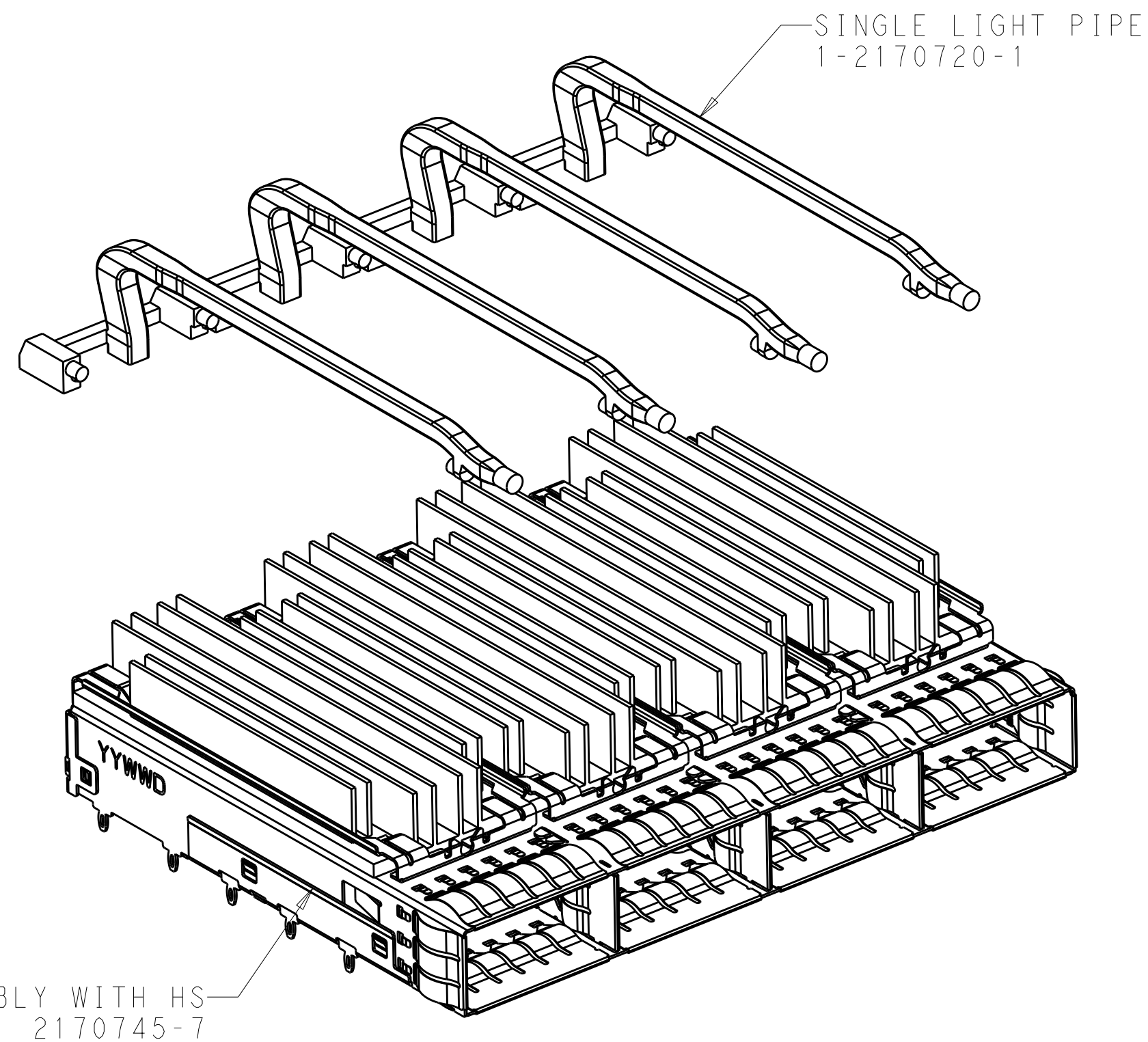
2170747-7 UNASSEMBLED CAGE ASSY WITH HS AND LIGHT PIPE ARE UNASSEMBLED, AND PACKAGED INDIVIDUALLY. CUSTOMIZED HEAT SINK SCALE 2:1
