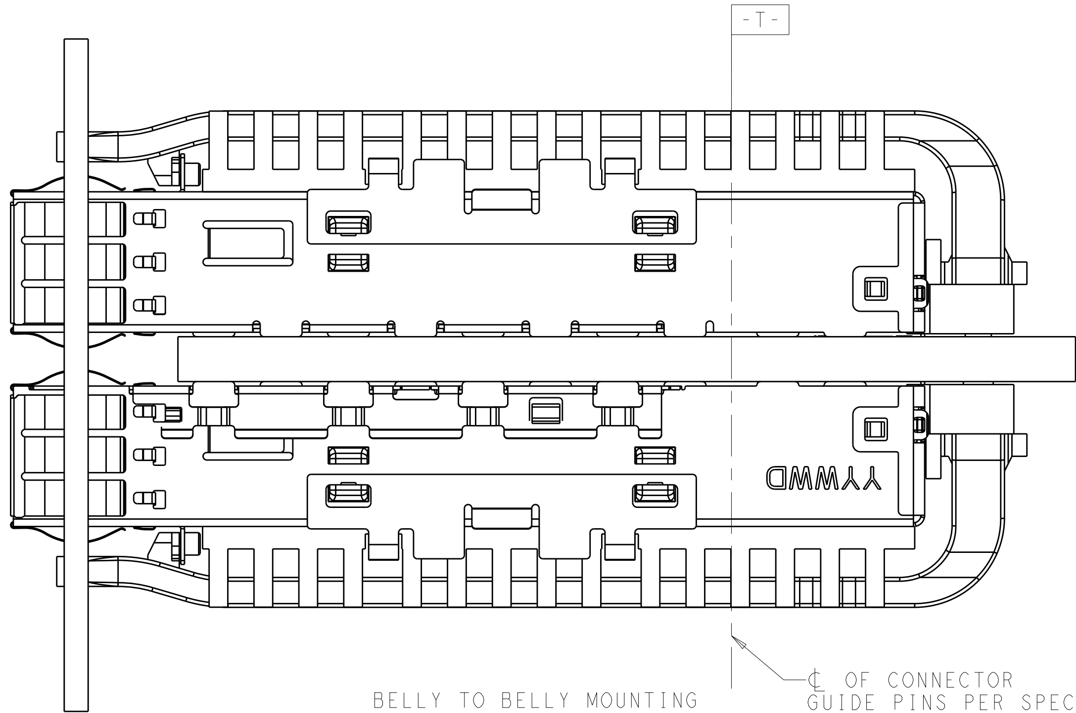
BELLY TO BELLY MOUNTING SCALE 4:1
