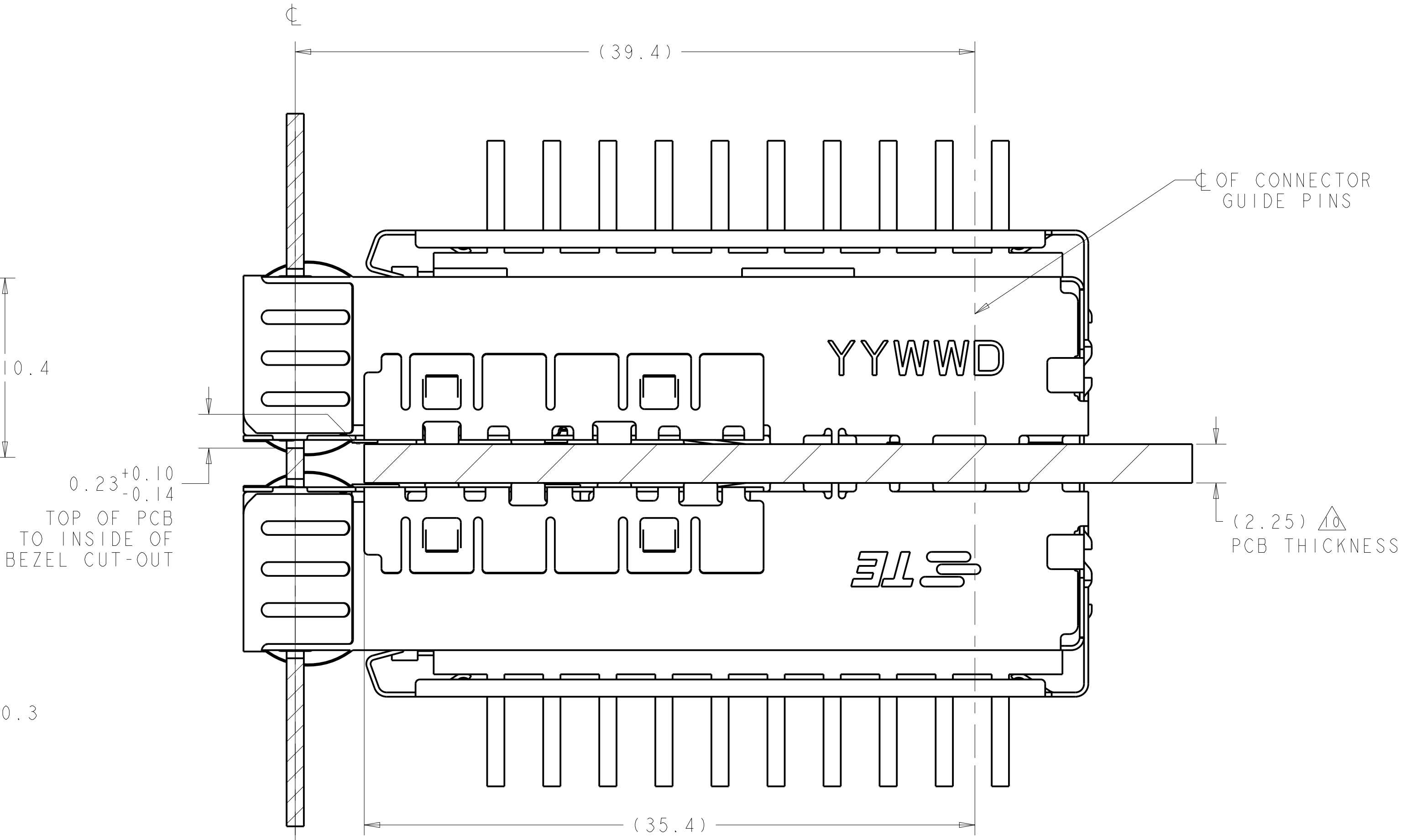
2149730 MOUNTED BELLY TO BELLY ON PC BOARD SHOWN THRU RECOMMENDED BEZEL
