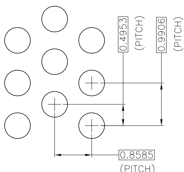
DETAIL N(20:1)
