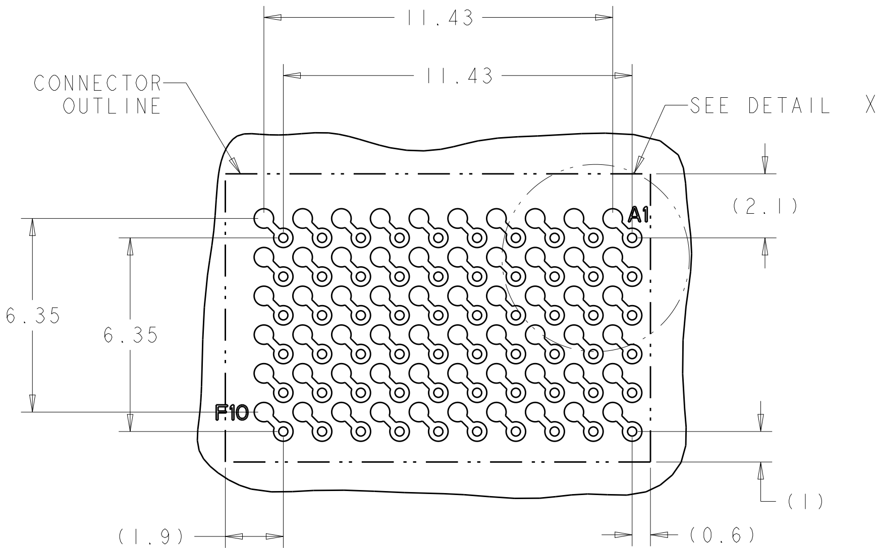
PCB LAYOUT (CONNECTOR SIDE) SCALE 8:1
