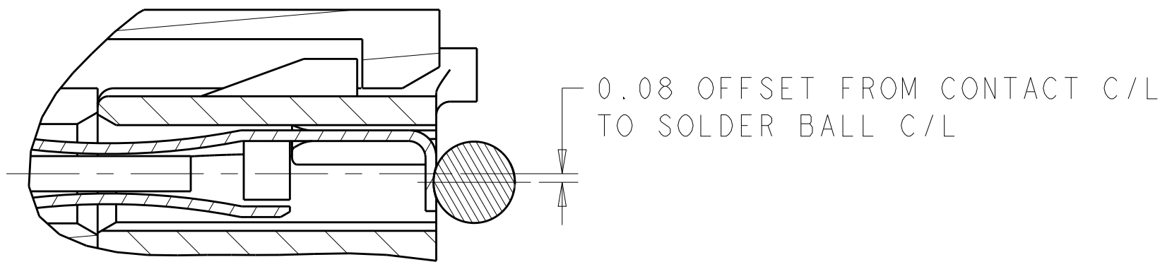
DETAIL T SCALE 20:1
